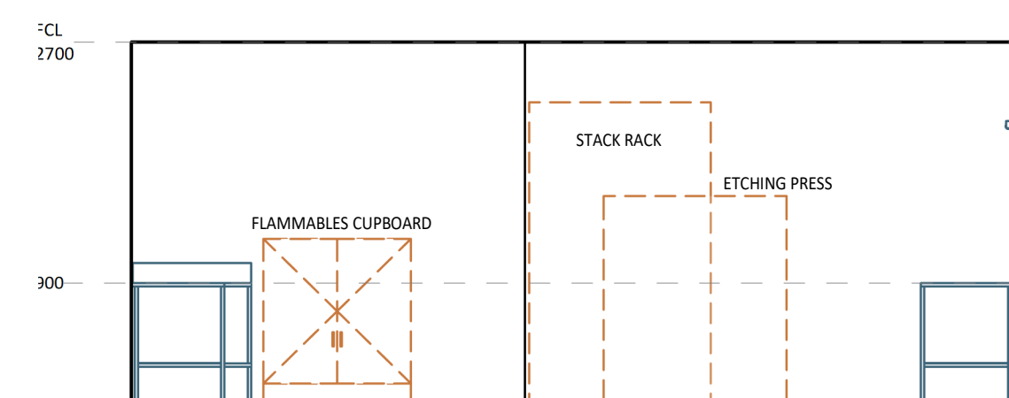
6 ELEVATION DETAIL 1 : 50
