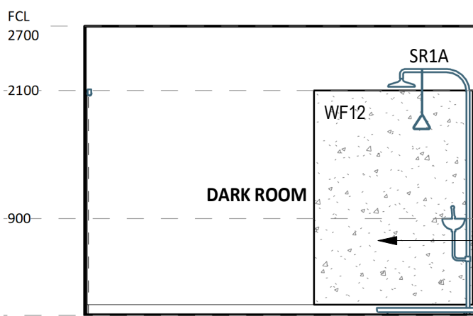
4 ELEVATION DETAIL 1 : 50
