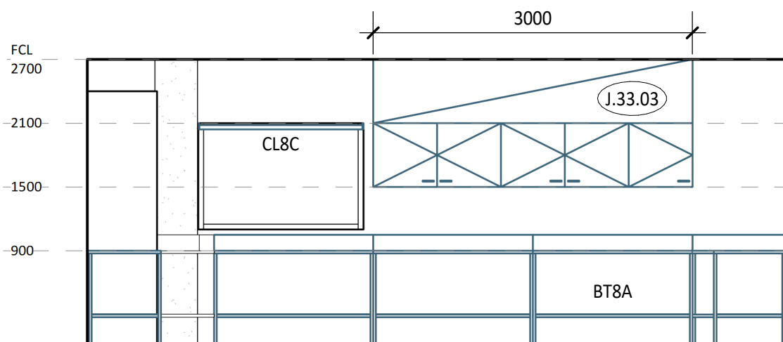
8 ELEVATION DETAIL 1 : 50
