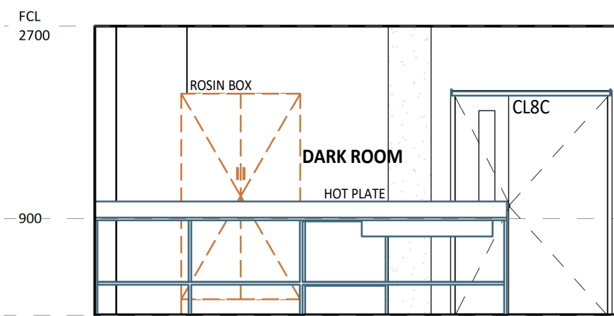
3 ELEVATION DETAIL 1 : 50
