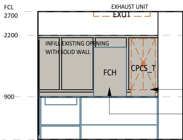
2 ELEVATION DETAIL 1 : 50
