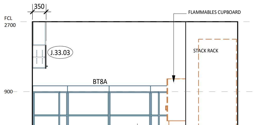
9 ELEVATION DETAIL 1 : 50
