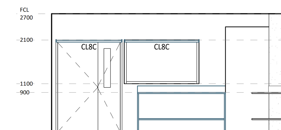
7 ELEVATION DETAIL 1 : 50
