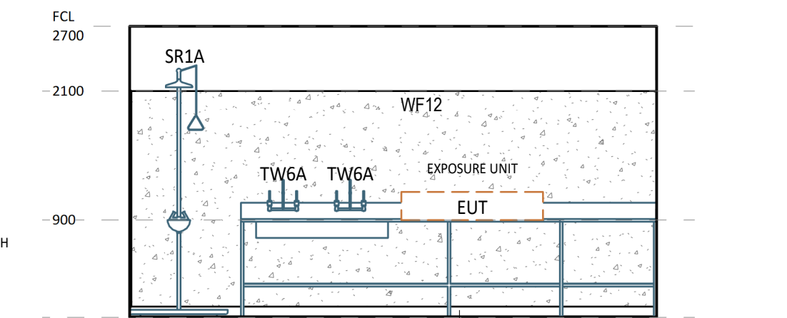
5 ELEVATION DETAIL 1 : 50
